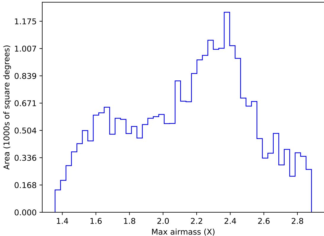
ddf_acor_sf25_lsf30_lsr10_v3.4_10yrs Yr 1 all bands: Max airmass
