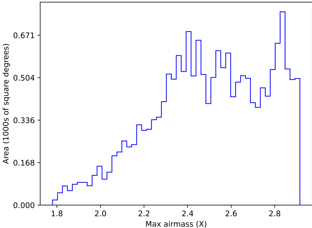
ddf_acor_sf25_lsf30_lsr10_v3.4_10yrs WFD z band: Max airmass
