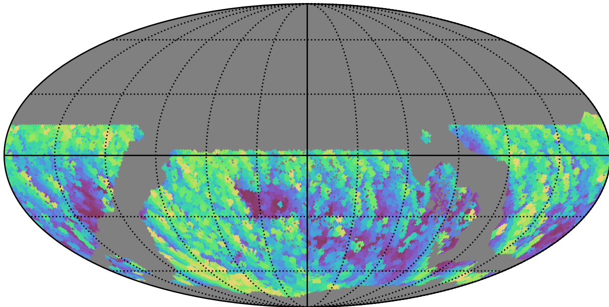
ddf_acor_sf25_lsf30_lsr10_v3.4_10yrs WFD y band: Max airmass
