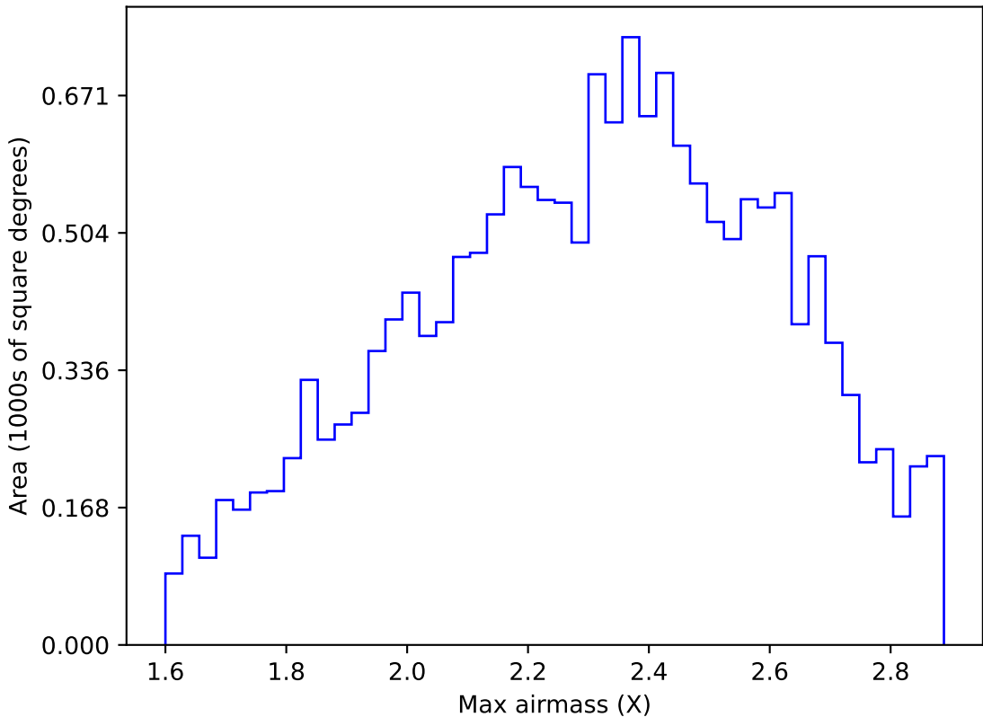
ddf_acor_sf25_ls30_lsr10_v3.4_10yrs WFD y band: Max airmass
