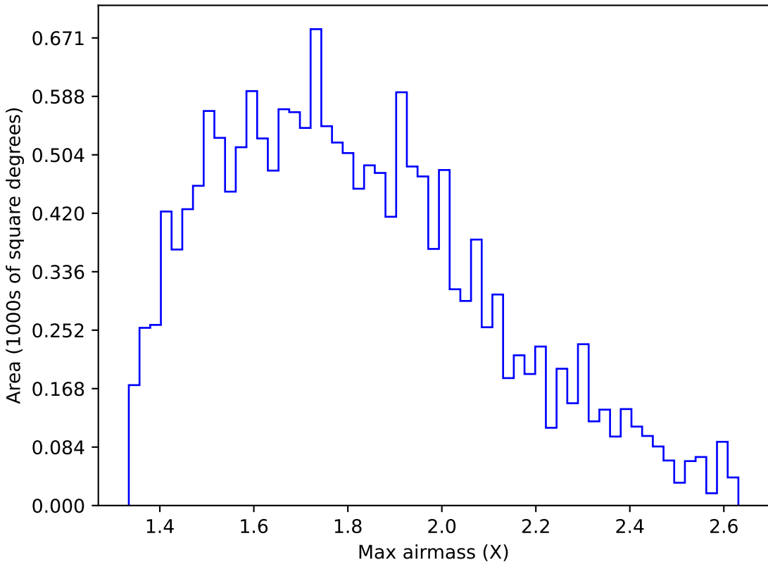
ddf_acor_sf25_lsf30_lsr10_v3.4_10yrs WFD u band: Max airmass
