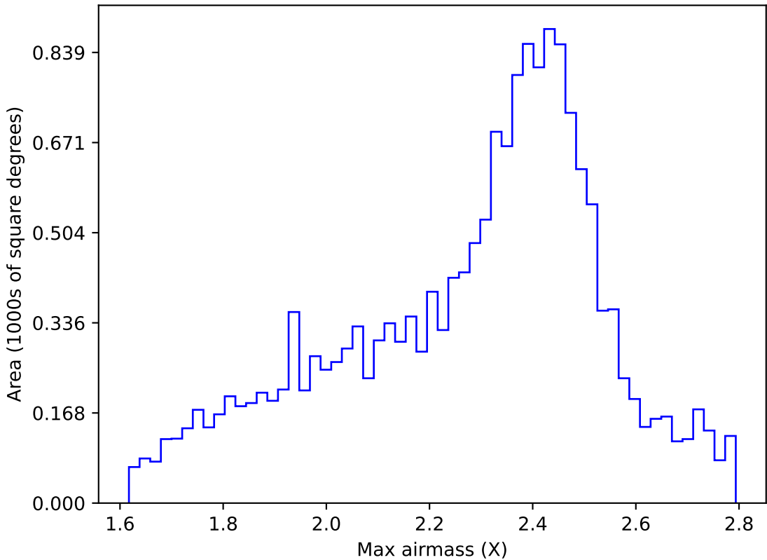
ddf_acor_sf25_lsf30_lsr10_v3.4_10yrs WFD r band: Max airmass
