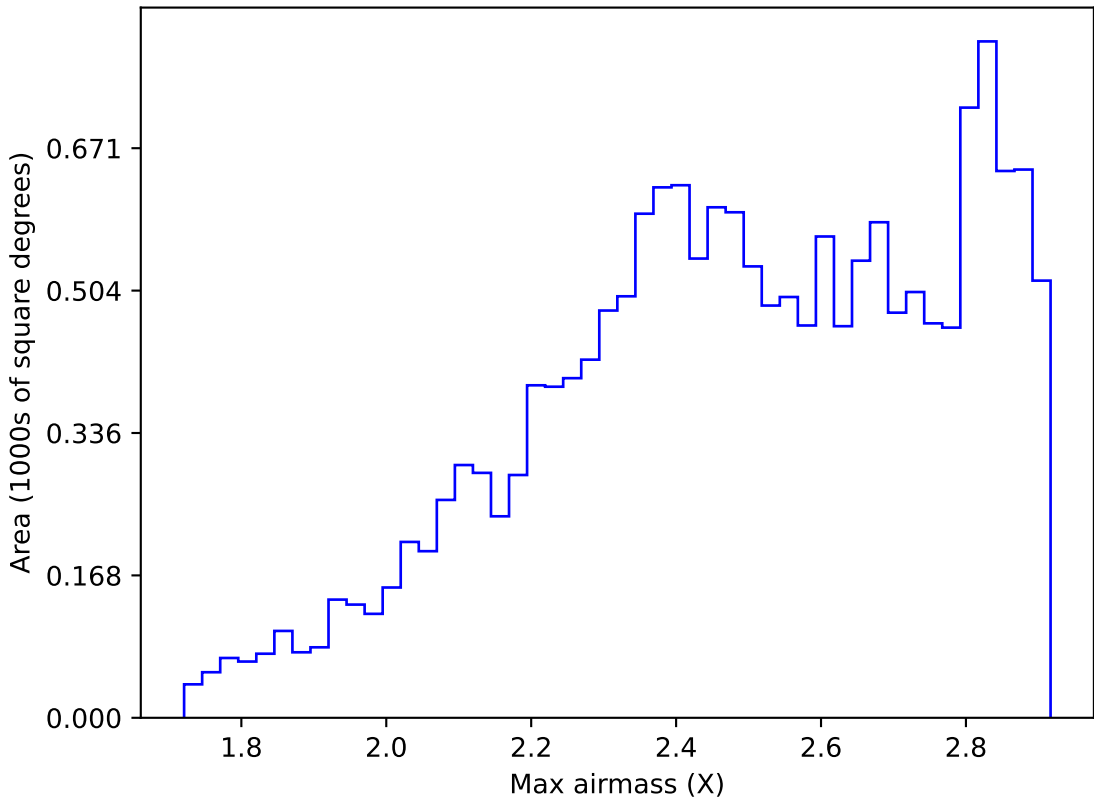
ddf_acor_sf25_lsf30_lsr10_v3.4_10yrs WFD i band: Max airmass
