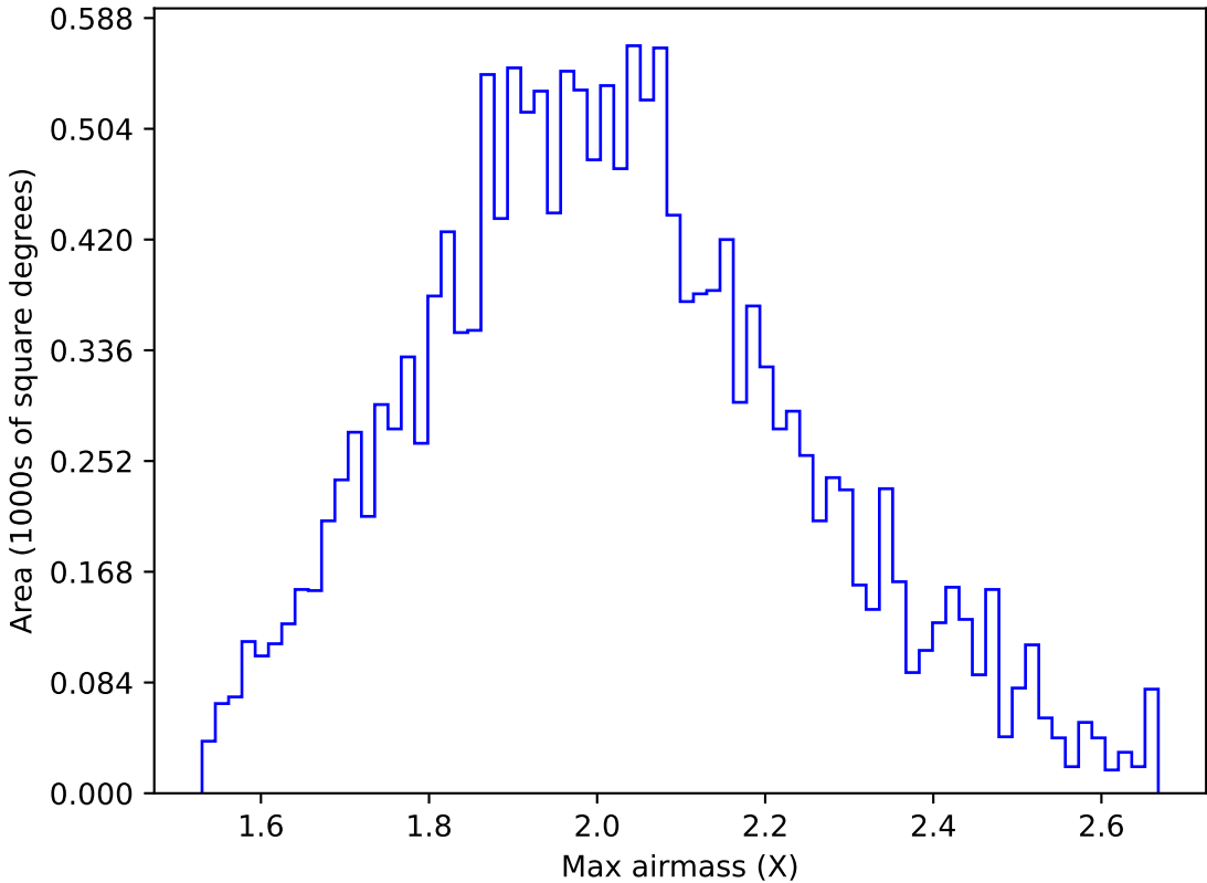
ddf_acor_sf25_lsf30_lsr10_v3.4_10yrs WFD g band: Max airmass
