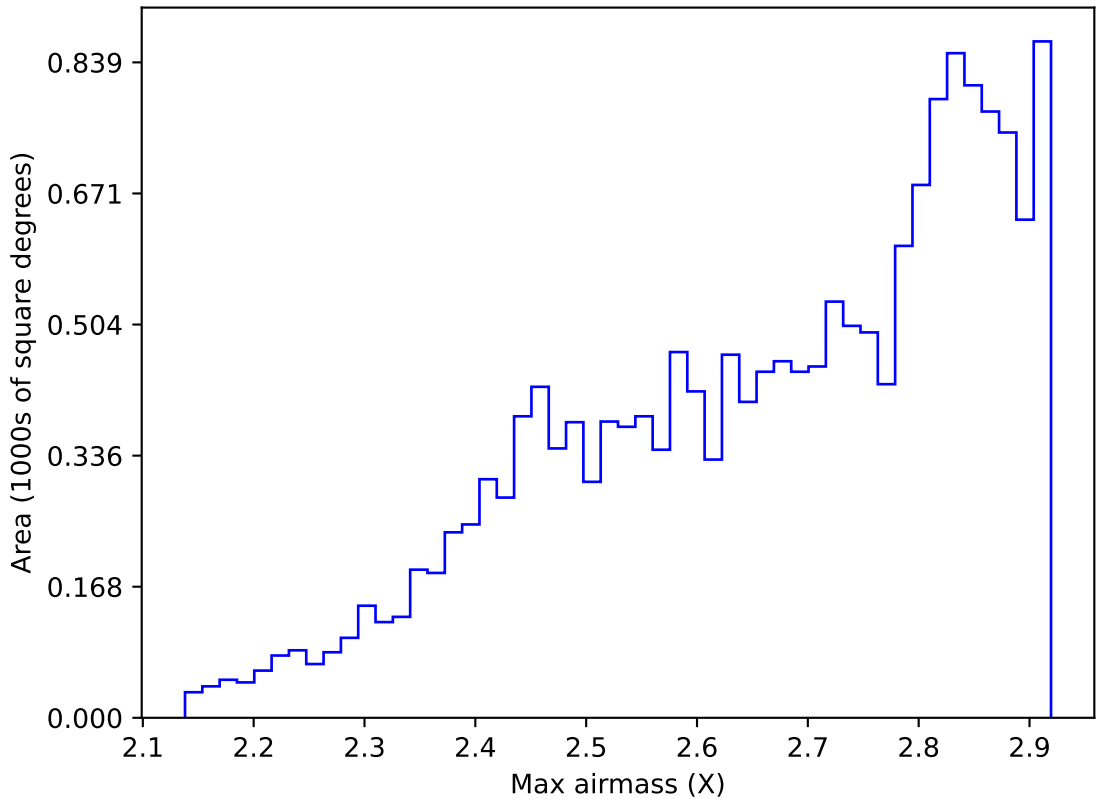
ddf_acor_sf25_lsf30_lsr10_v3.4_10yrs WFD all bands: Max airmass
