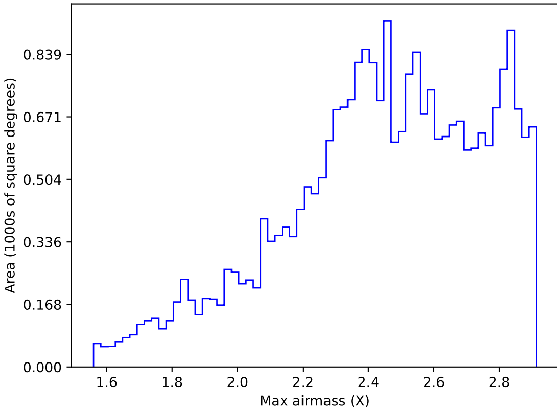
ddf_acor_sf25_lsf30_lsr10_v3.4_10yrs All sky z band: Max airmass
