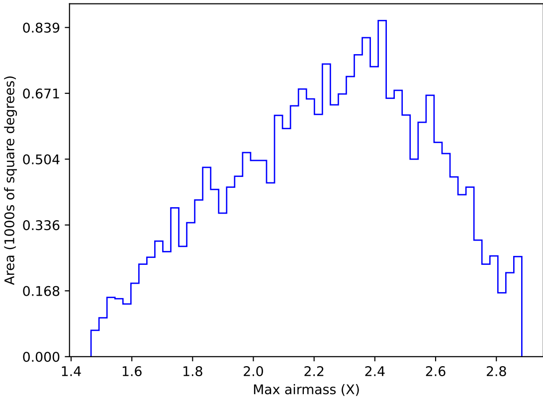
ddf_acor_sf25_lsf30_lsr10_v3.4_10yrs All sky y band: Max airmass
