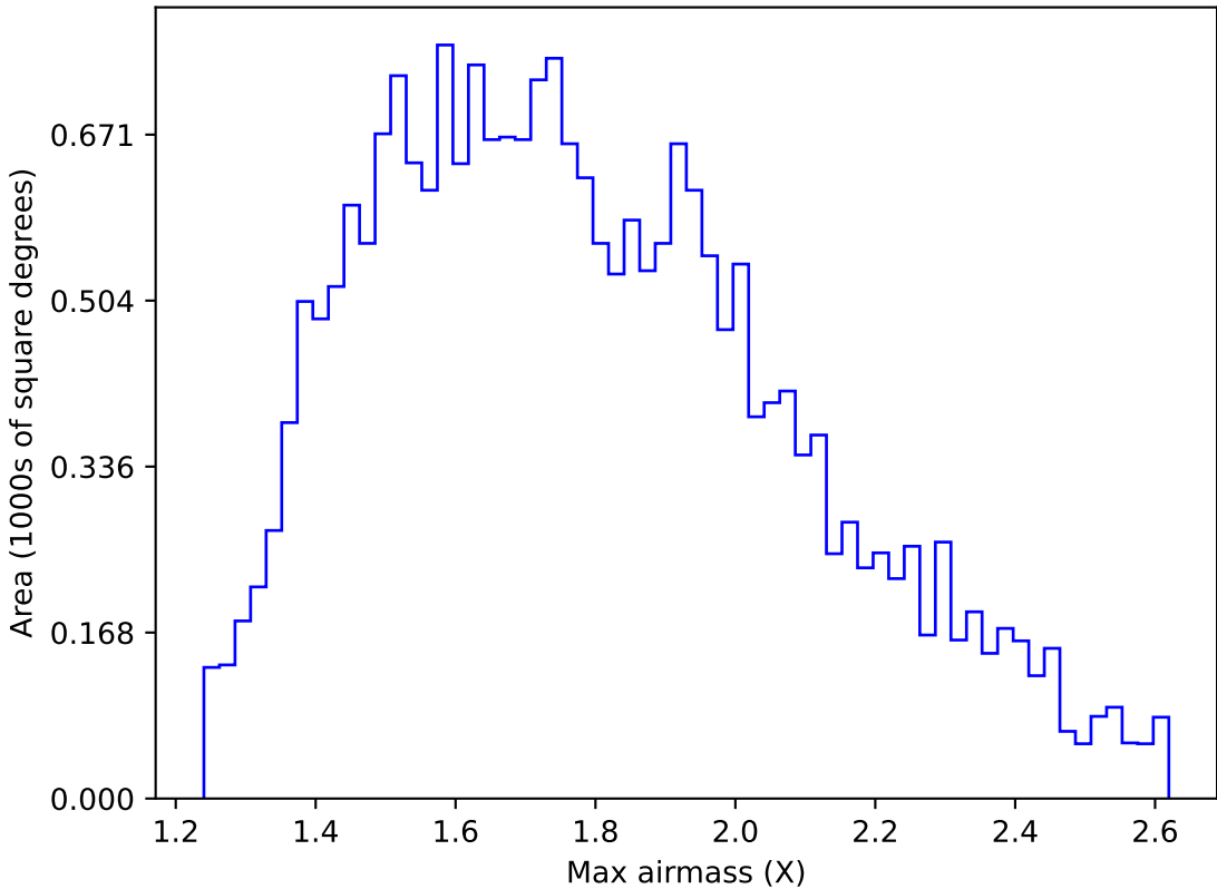
ddf_acor_sf25_lsf30_lsr10_v3.4_10yrs All sky u band: Max airmass
