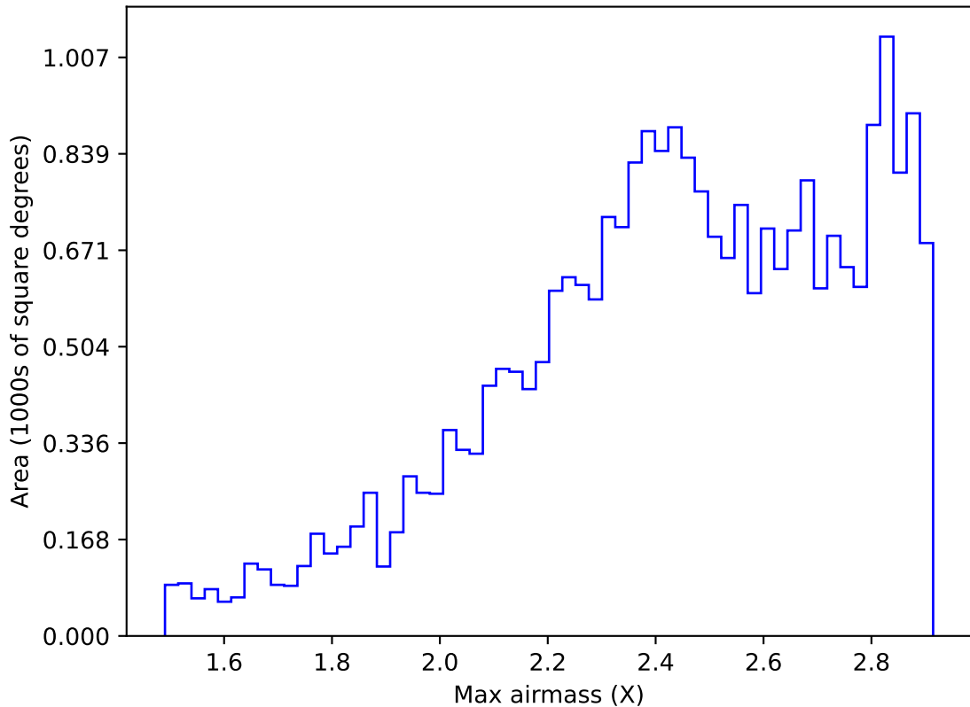
ddf_acor_sf25_lsf30_lsr10_v3.4_10yrs All sky i band: Max airmass
