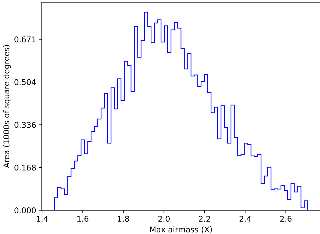
ddf_acor_sf25_lsf30_lsr10_v3.4_10yrs All sky g band: Max airmass
