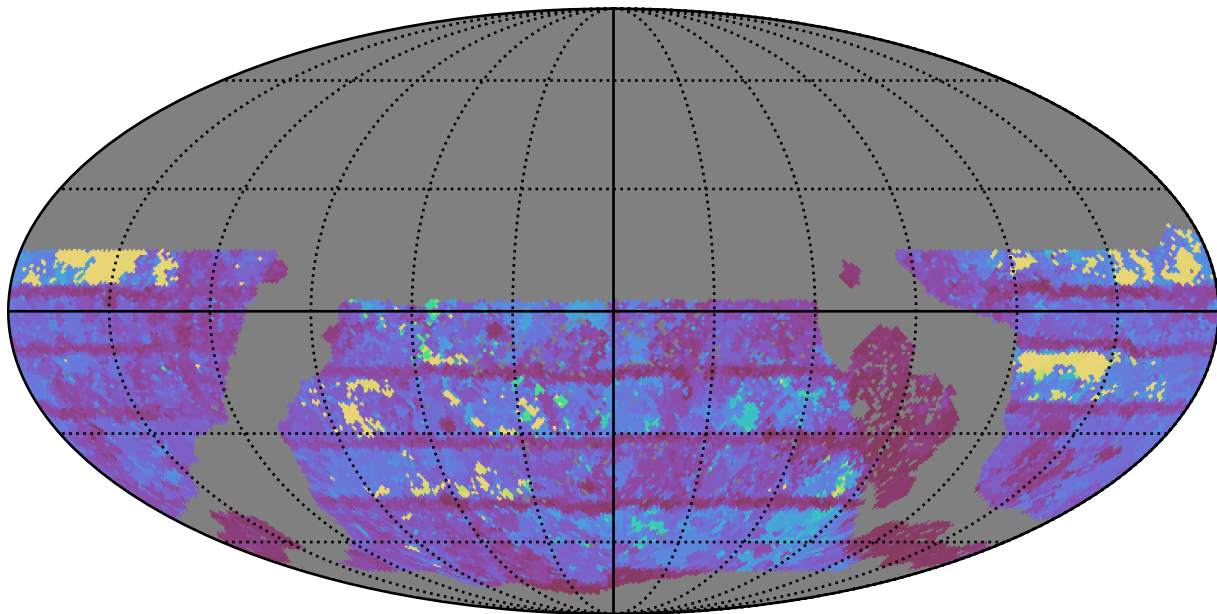
ddf_acor_sf25_lsf30_lsr10_v3.4_10yrs WFD r band: Max Inter-Night Gap
