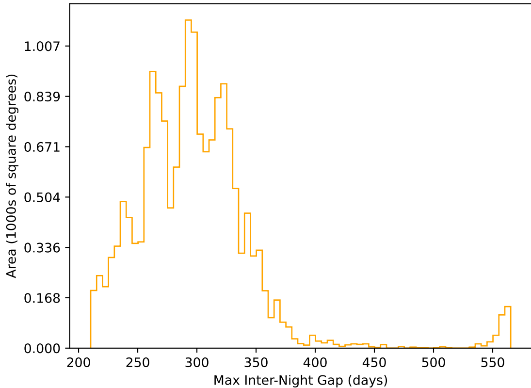
ddf_acor_sf25_lsf30_lsr10_v3.4_10yrs WFD r band: Max Inter-Night Gap
