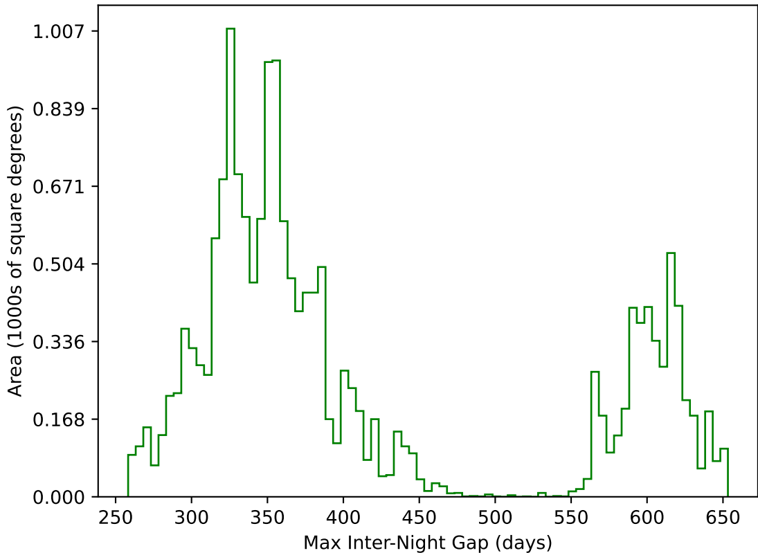
ddf_acor_sf25_lsf30_lsr10_v3.4_10yrs WFD g band: Max Inter-Night Gap
