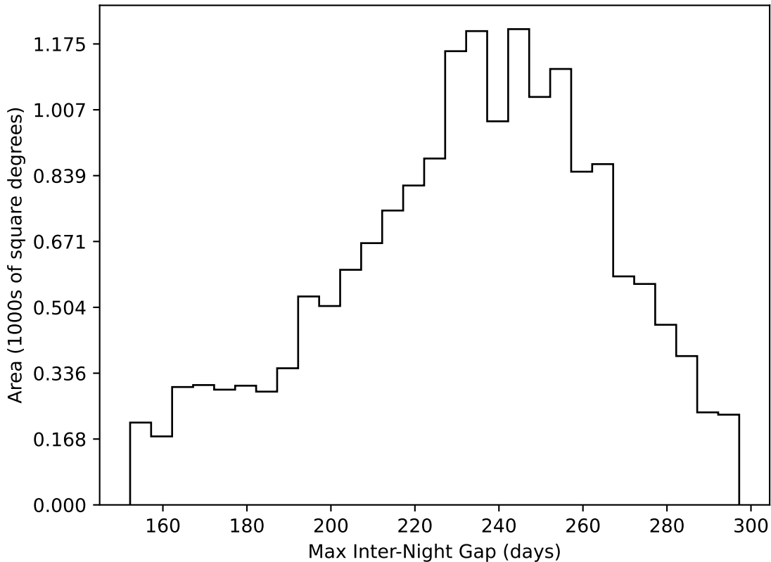
ddf_acor_sf25_lsf30_lsr10_v3.4_10yrs WFD all bands: Max Inter-Night Gap
