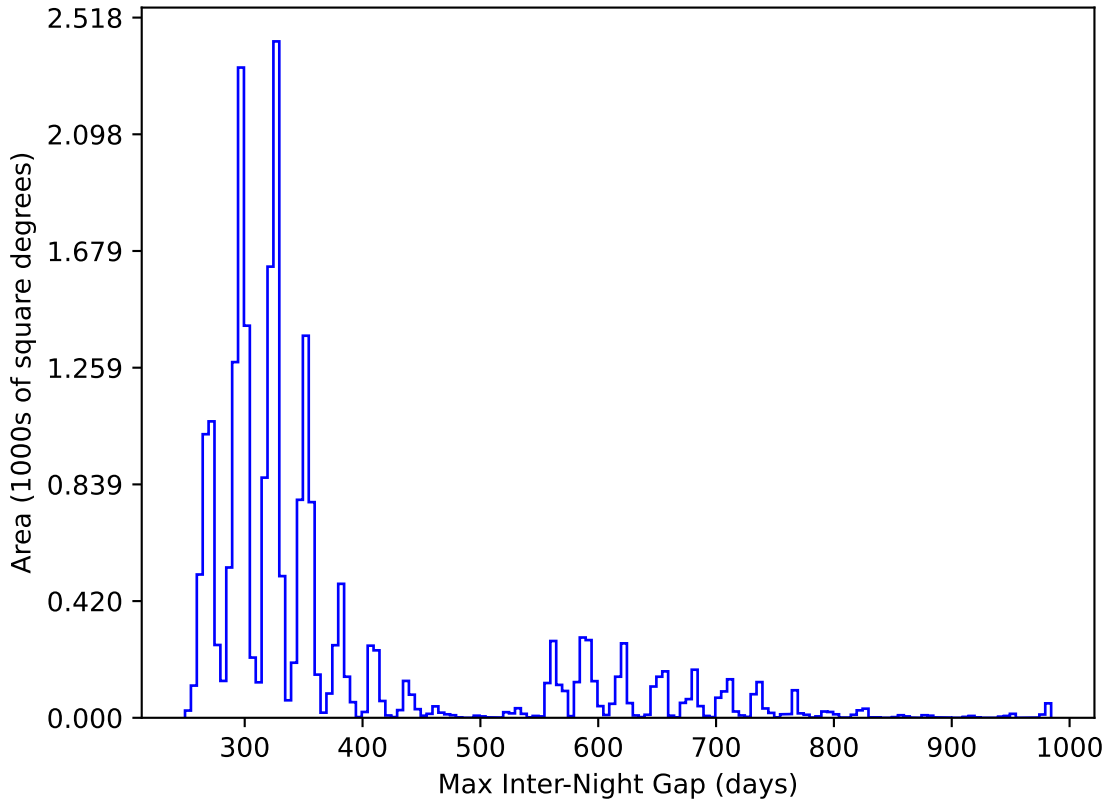
ddf_acor_sf25_lsf30_lsr10_v3.4_10yrs All sky y band: Max Inter-Night Gap
