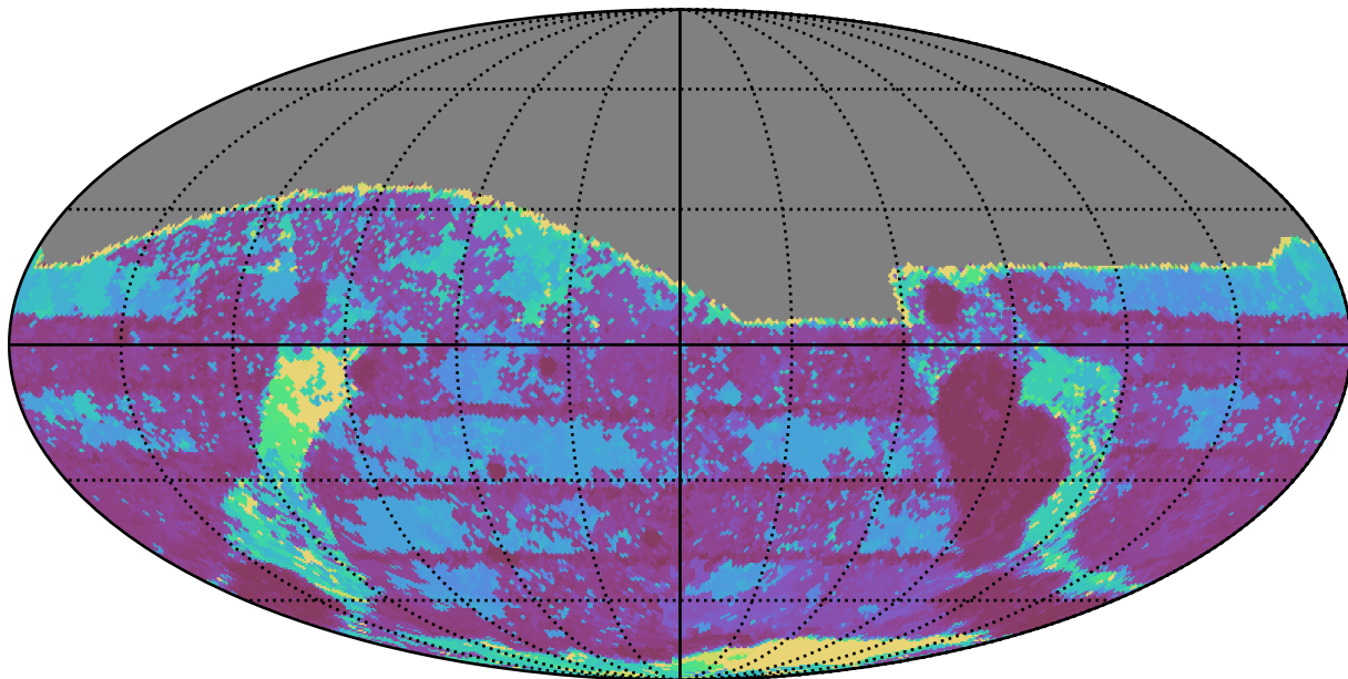
ddf_acor_sf25_lsf30_lsr10_v3.4_10yrs All sky g band: Max Inter-Night Gap
