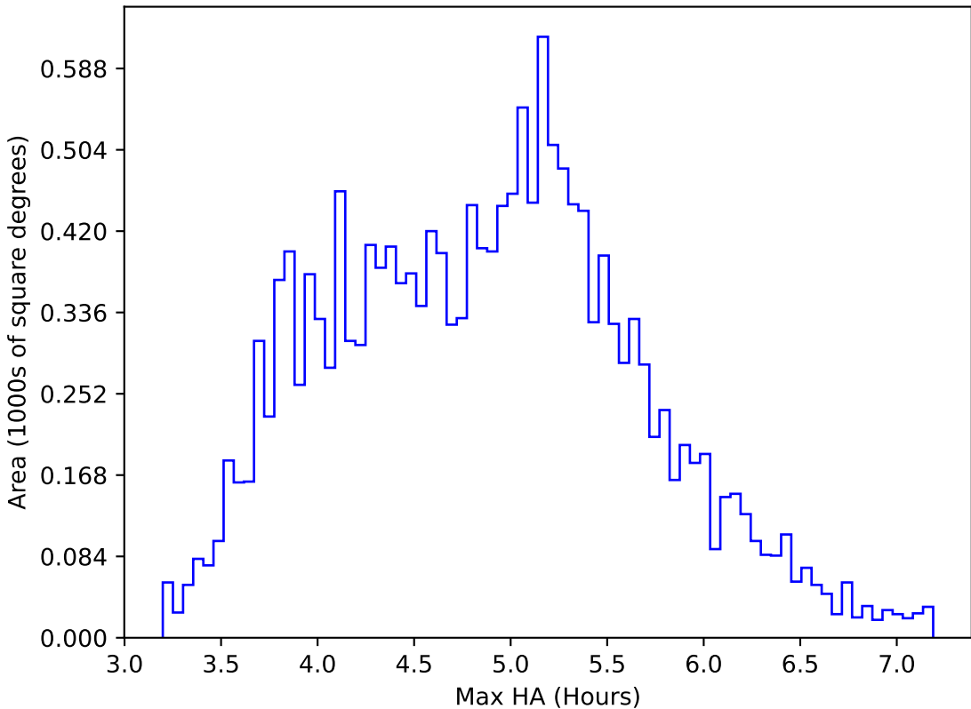
ddf_acor_sf25_lsf30_lsr10_v3.4_10yrs WFD z band: Max HA
