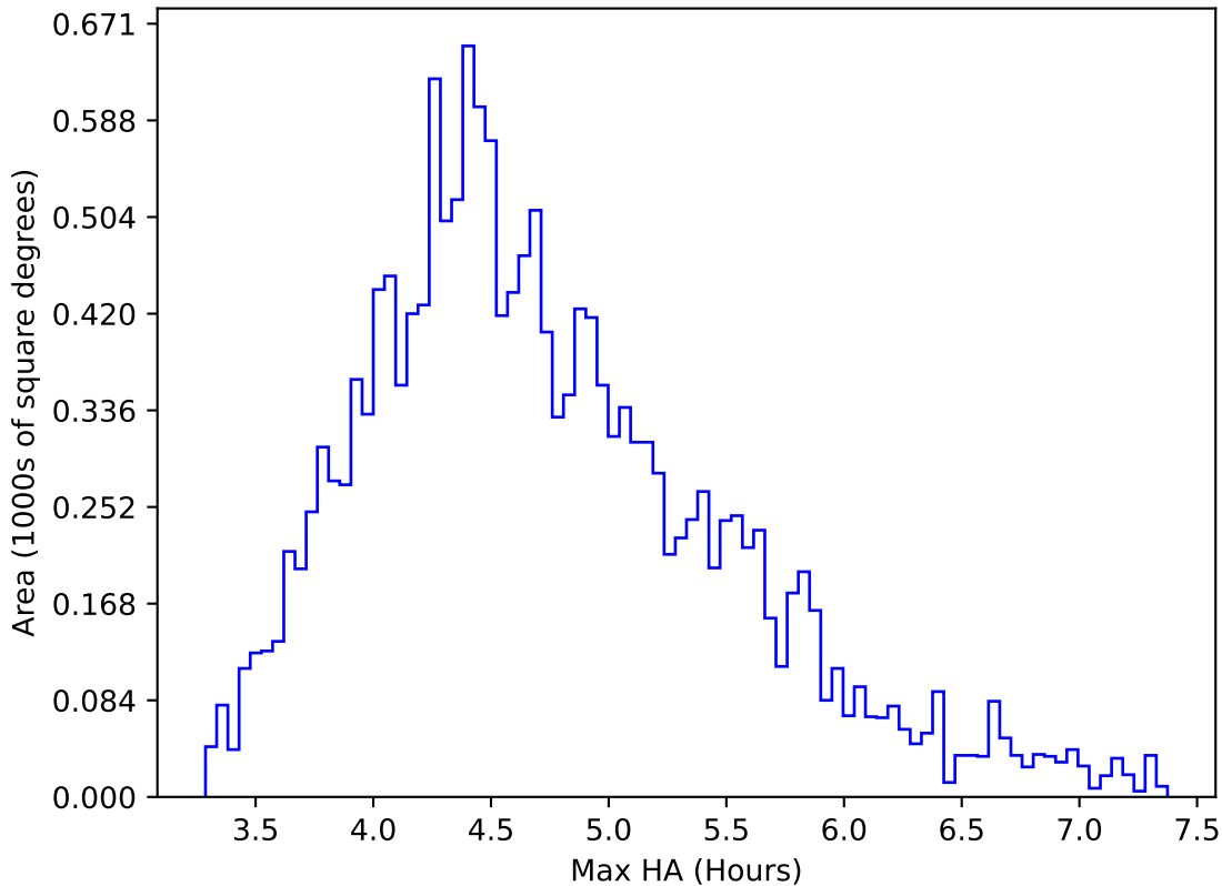
ddf_acor_sf25_lsf30_lsr10_v3.4_10yrs WFD y band: Max HA
