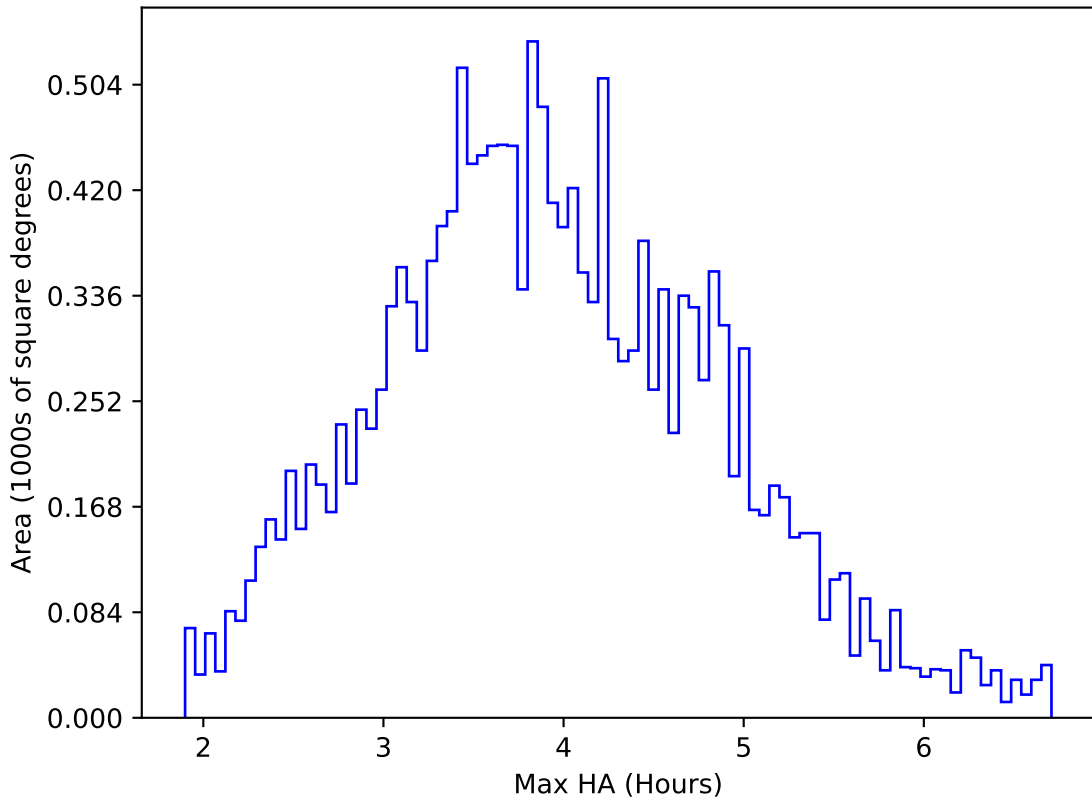
ddf_acor_sf25_lsf30_lsr10_v3.4_10yrs WFD u band: Max HA
