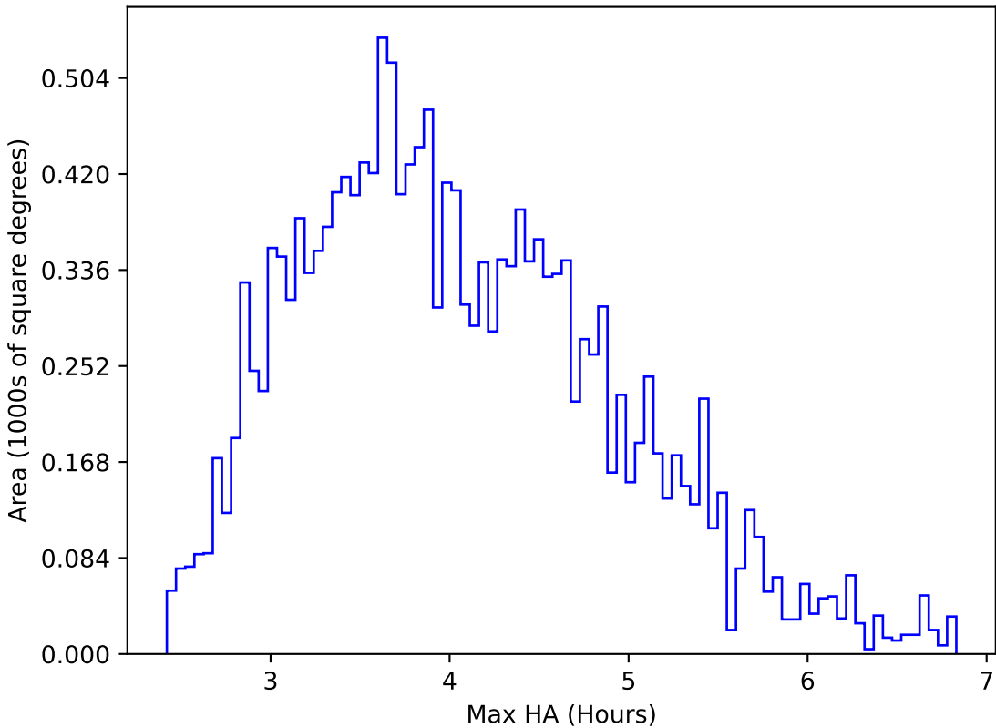
ddf_acor_sf25_lsf30_lsr10_v3.4_10yrs WFD g band: Max HA
