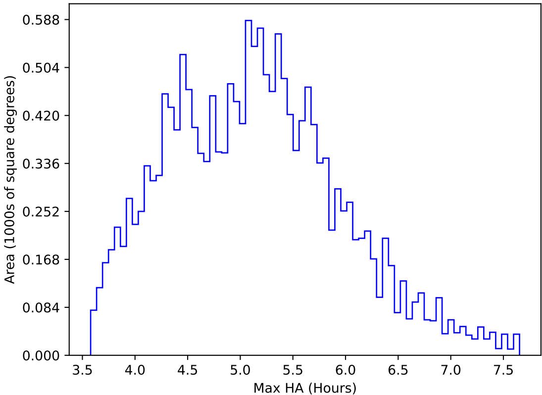
ddf_acor_sf25_lsf30_lsr10_v3.4_10yrs WFD all bands: Max HA
