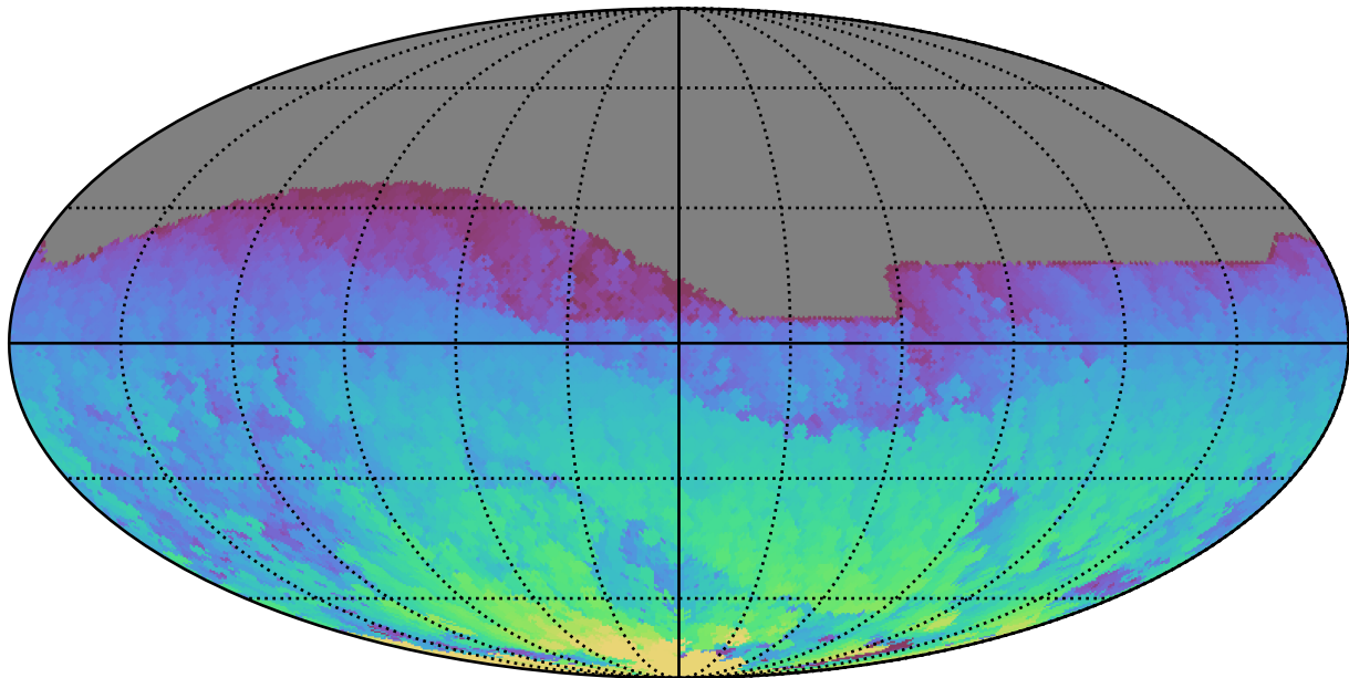
ddf_acor_sf25_lsf30_lsr10_v3.4_10yrs All sky z band: Max HA
