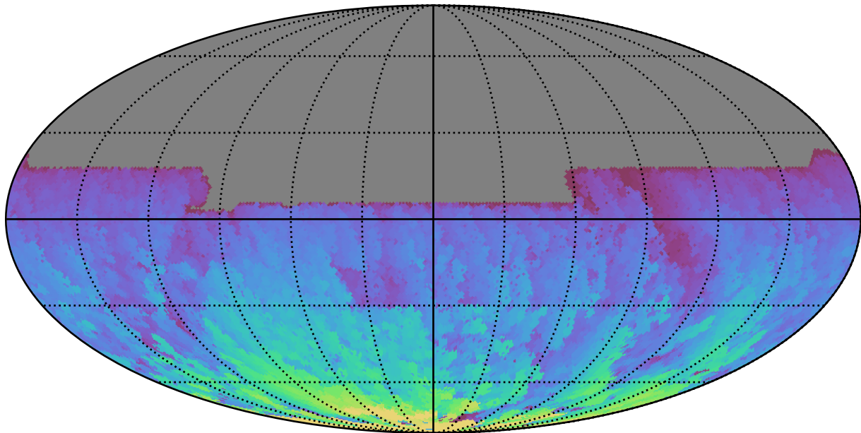
ddf_acor_sf25_lsf30_lsr10_v3.4_10yrs All sky y band: Max HA
