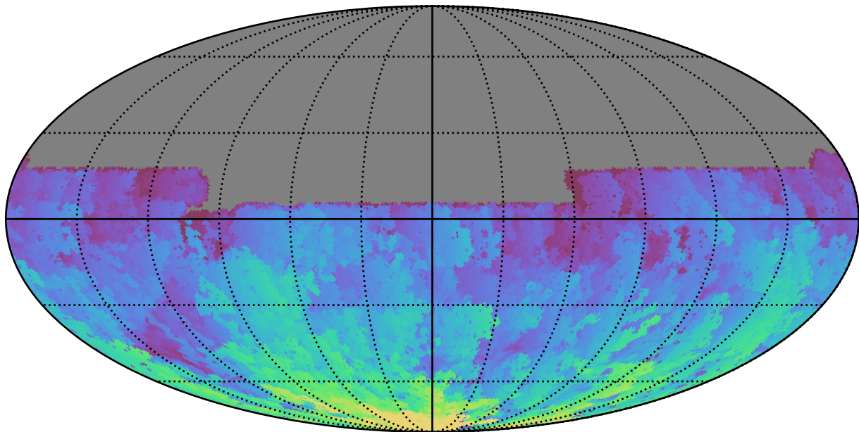
ddf_acor_sf25_lsf30_lsr10_v3.4_10yrs All sky u band: Max HA
