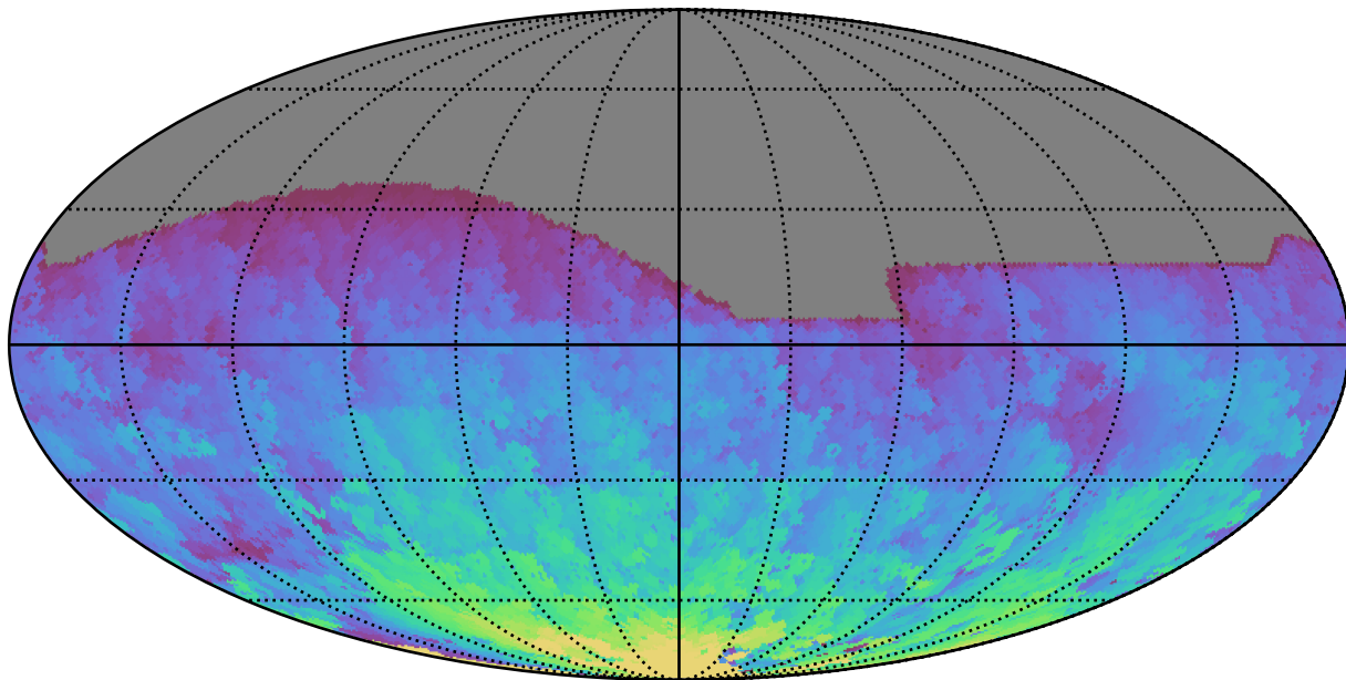
ddf_acor_sf25_lsf30_lsr10_v3.4_10yrs All sky r band: Max HA
