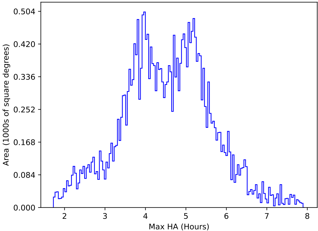
ddf_acor_sf25_lsf30_lsr10_v3.4_10yrs All sky i band: Max HA
