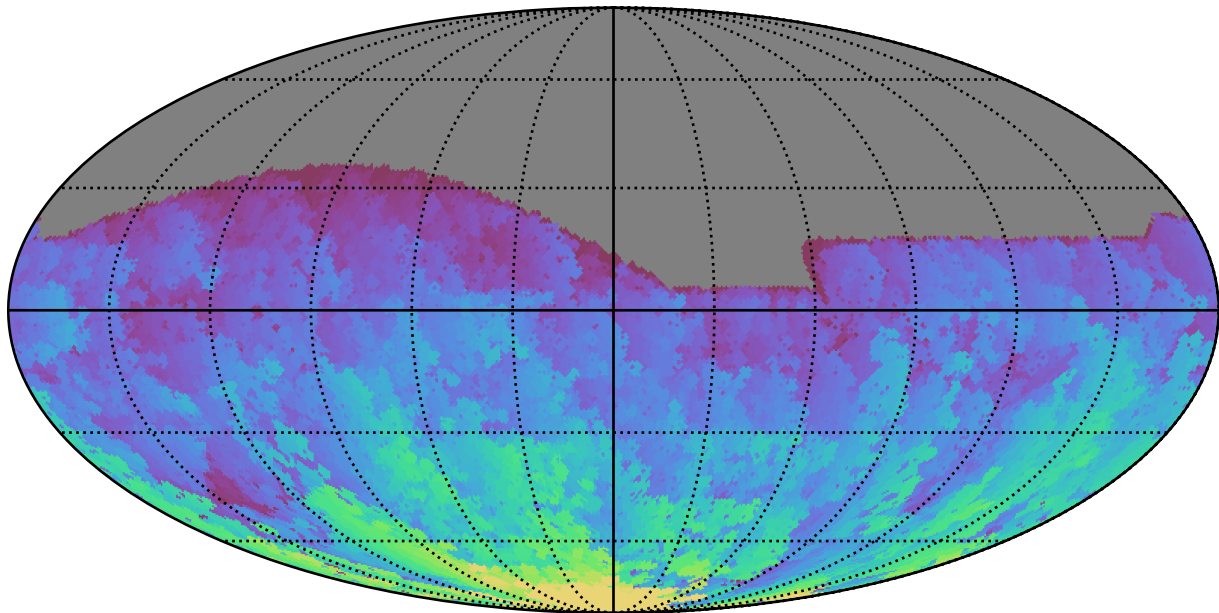
ddf_acor_sf25_lsf30_lsr10_v3.4_10yrs All sky g band: Max HA
