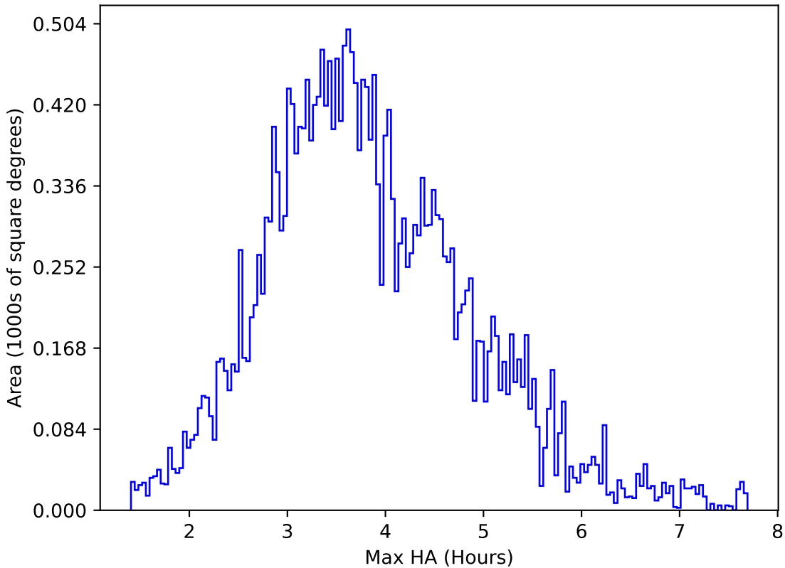
ddf_acor_sf25_lsf30_lsr10_v3.4_10yrs All sky g band: Max HA
