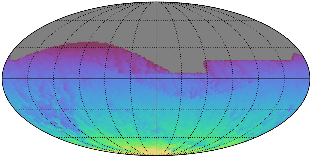
ddf_acor_sf25_lsf30_lsr10_v3.4_10yrs All sky all bands: Max HA
