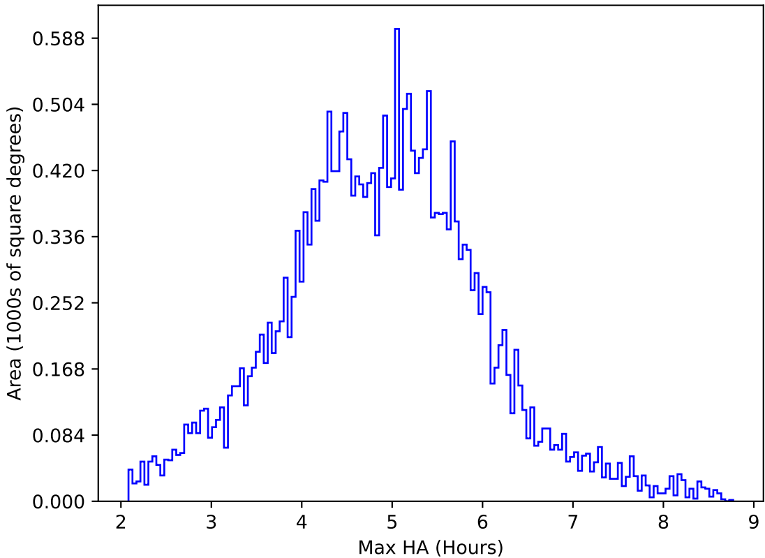
ddf_acor_sf25_lsf30_lsr10_v3.4_10yrs All sky all bands: Max HA
