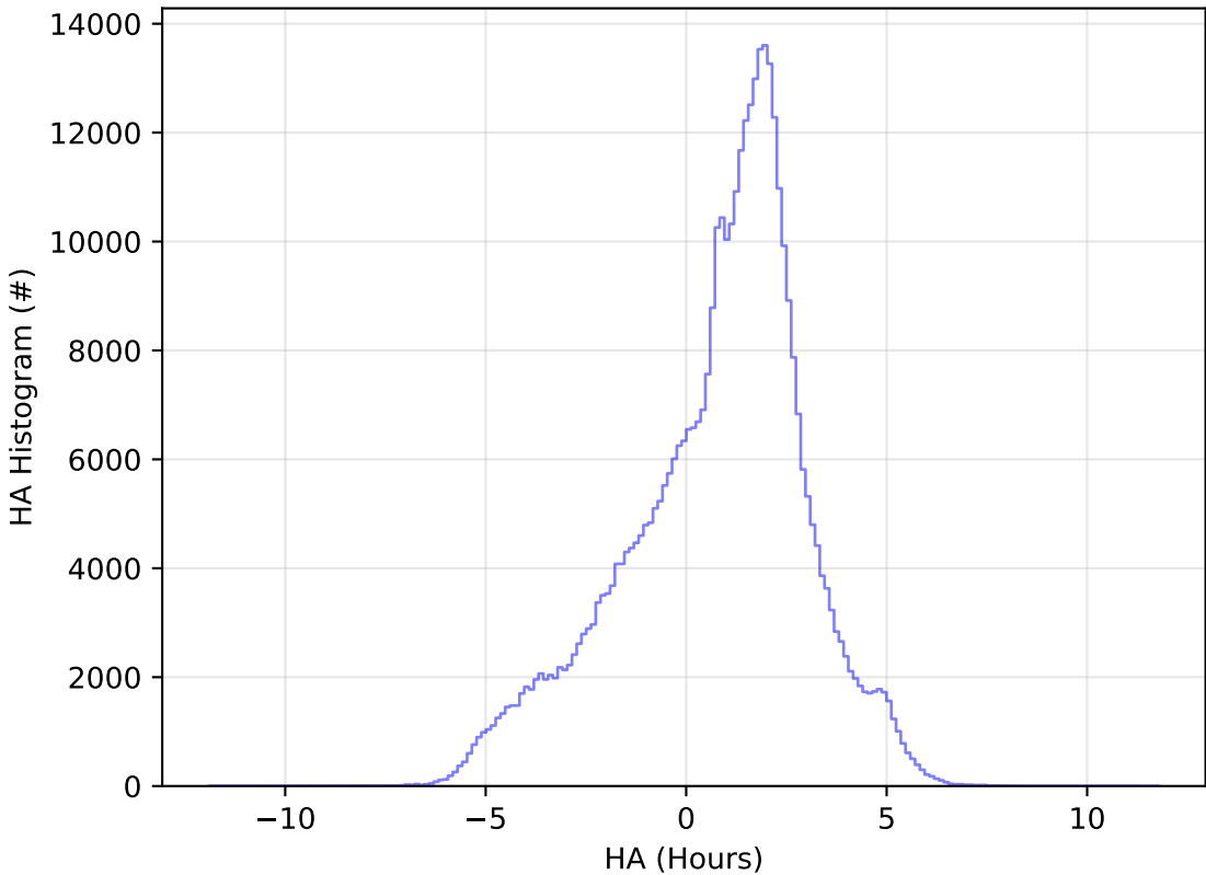
ddf_acor_sf25_lsf30_lsr10_v3.4_10yrs WFD z band: HA Histogram
