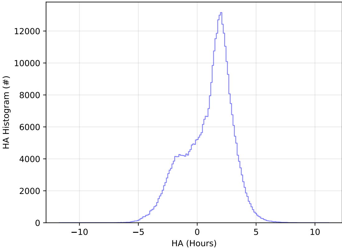
ddf_acor_sf25_lsf30_lsr10_v3.4_10yrs WFD y band: HA Histogram
