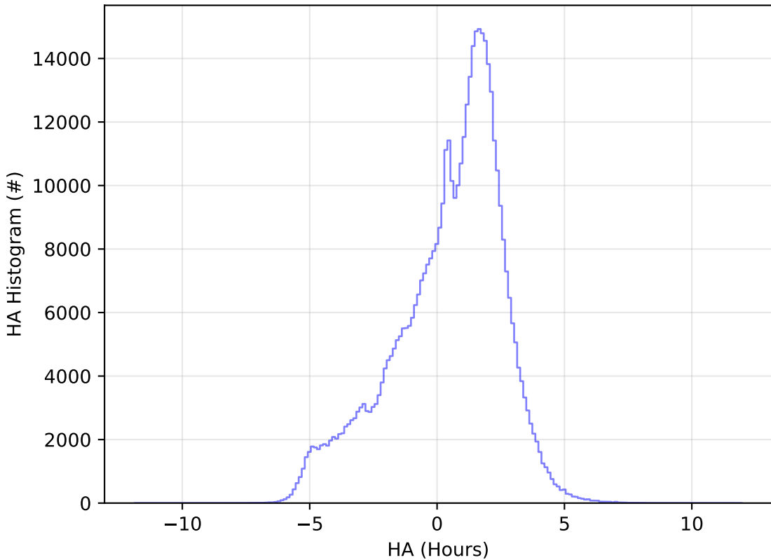
ddf_acor_sf25_lsf30_lsr10_v3.4_10yrs WFD r band: HA Histogram
