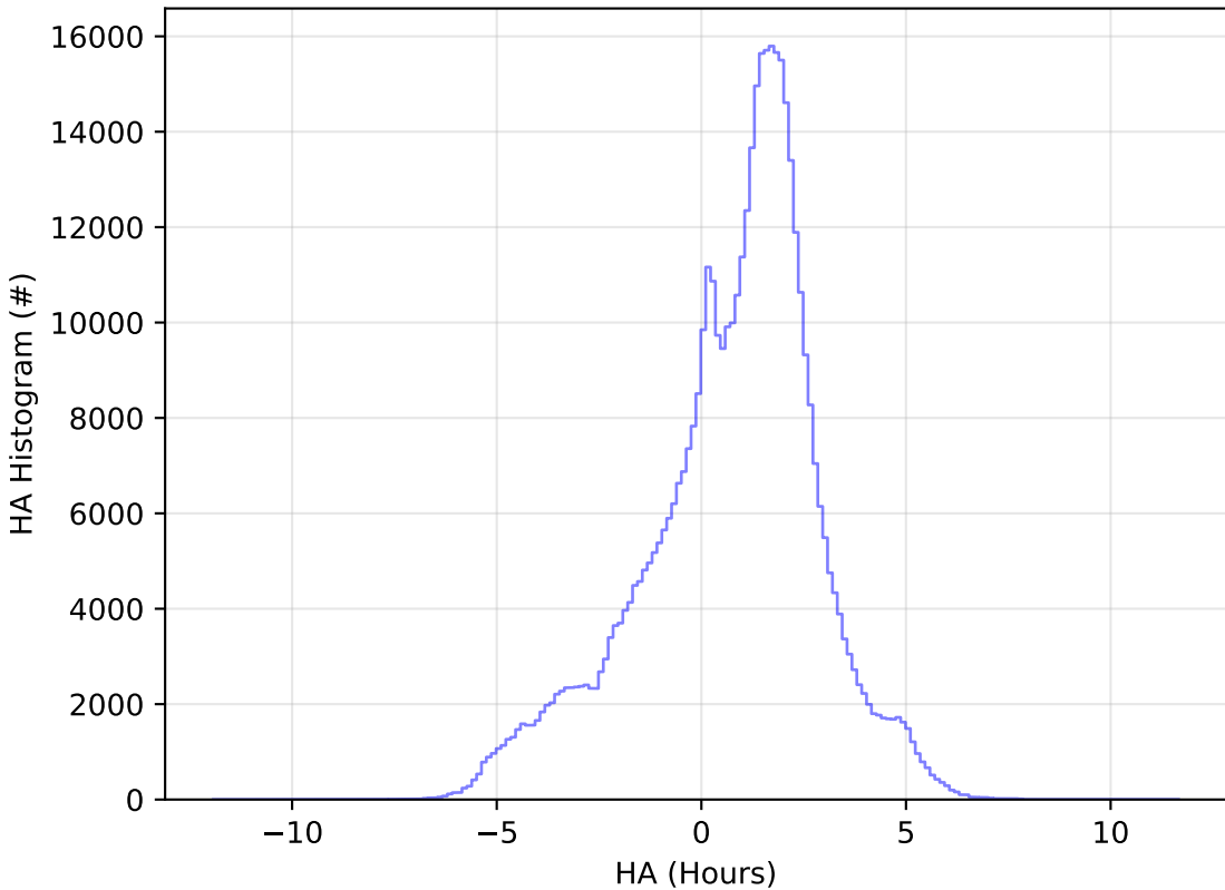
ddf_acor_sf25_lsf30_lsr10_v3.4_10yrs WFD i band: HA Histogram
