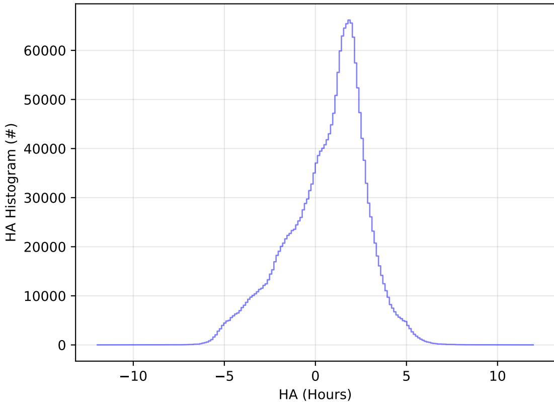
ddf_acor_sf25_lsf30_lsr10_v3.4_10yrs WFD all bands: HA Histogram
