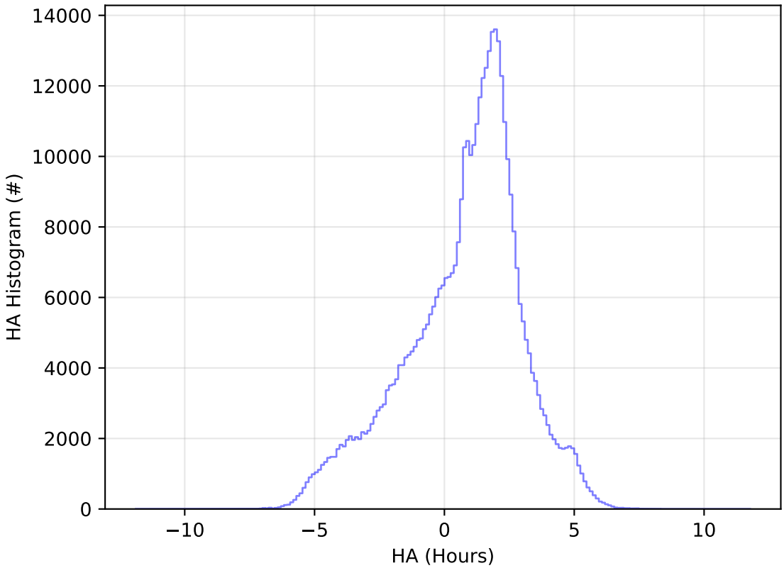
ddf_acor_sf25_lsf30_lsr10_v3.4_10yrs All sky z band: HA Histogram
