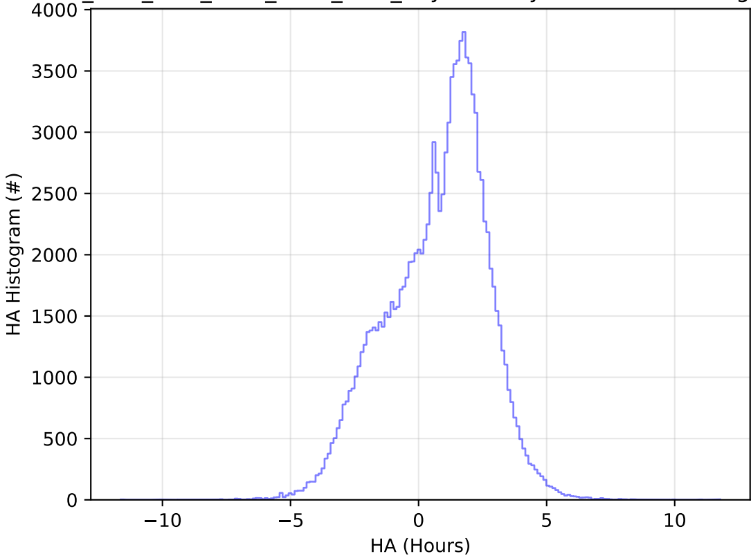
ddf_acor_sf25_lsf30_lsr10_v3.4_10yrs All sky u band: HA Histogram
