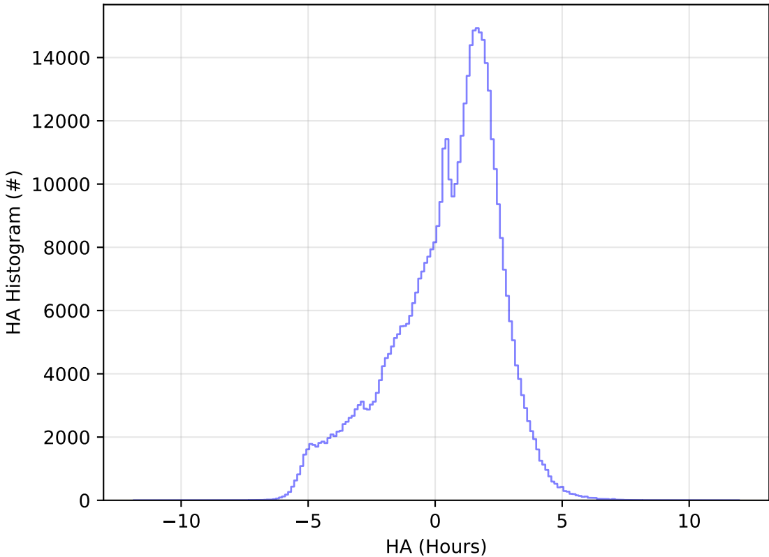
ddf_acor_sf25_lsf30_lsr10_v3.4_10yrs All sky r band: HA Histogram
