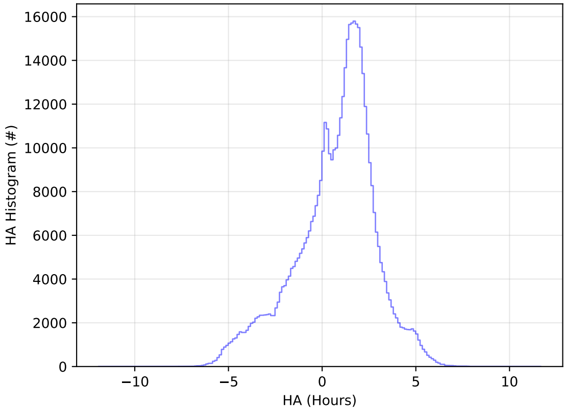
ddf_acor_sf25_lsf30_lsr10_v3.4_10yrs All sky i band: HA Histogram
