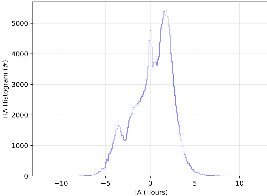
ddf_acor_sf25_lsf30_lsr10_v3.4_10yrs All sky g band: HA Histogram
