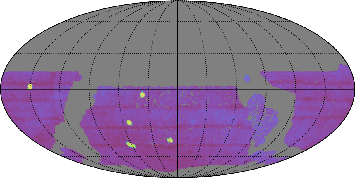
ddf_acor_sf25_lsf30_lsr10_v3.4_10yrs gri WFD: Fraction of visits with a revisit < 60 min
