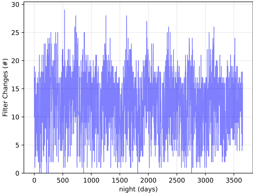
ddf_acor_sf25_lsf30_lsr10_v3.4_10yrs Per Night: Filter Changes
