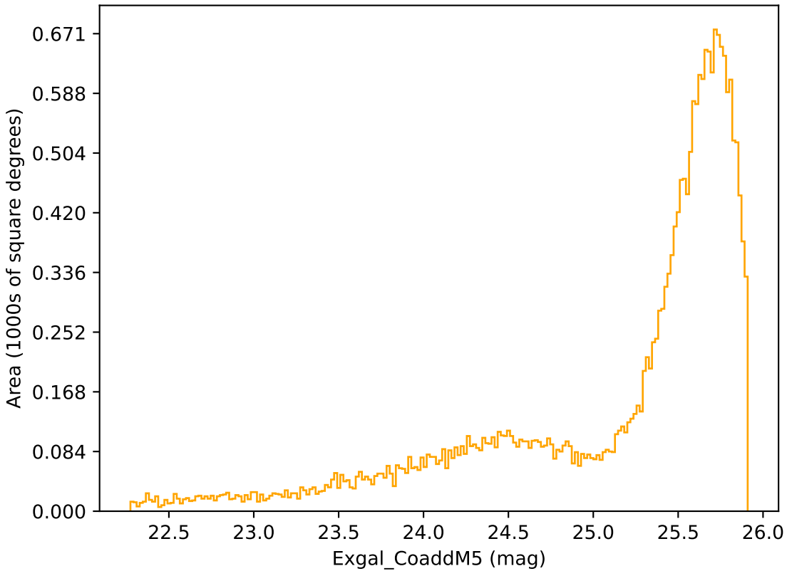
ddf_acor_sf25_lsf30_lsr10_v3.4_10yrs Yr 1 r band: Exgal_CoaddM5
