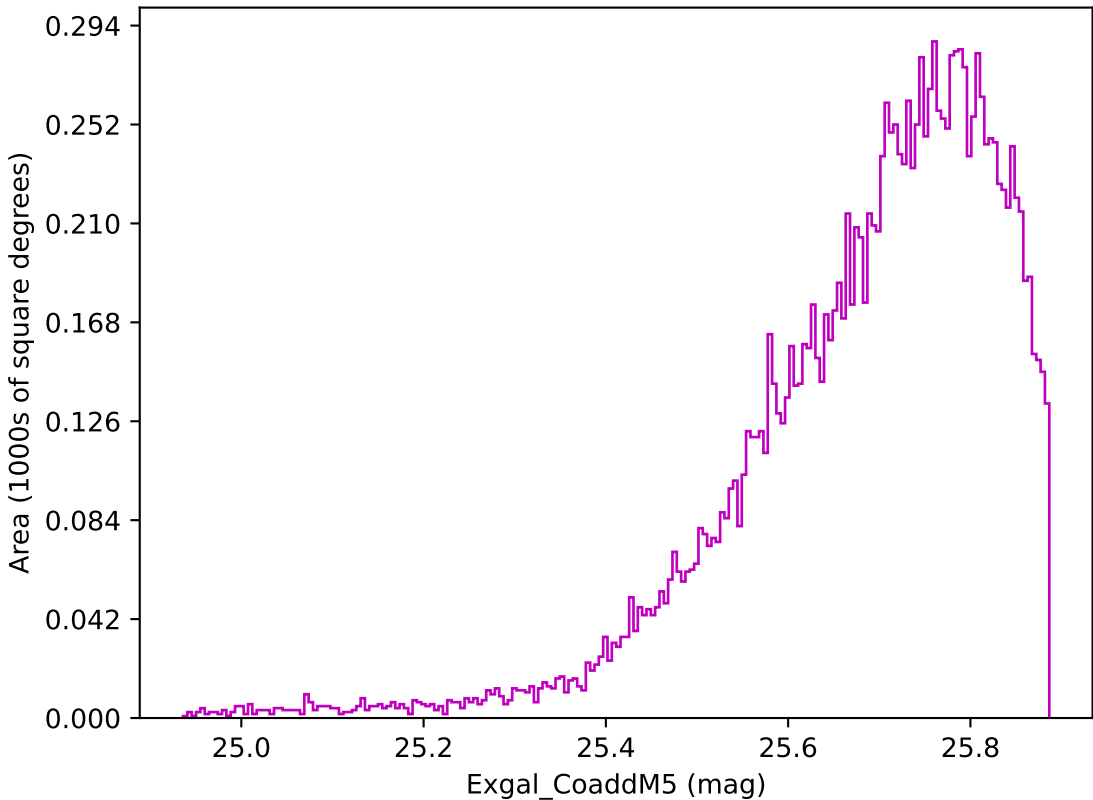
ddf_acor_sf25_lsf30_lsr10_v3.4_10yrs WFD z band: Exgal_CoaddM5
