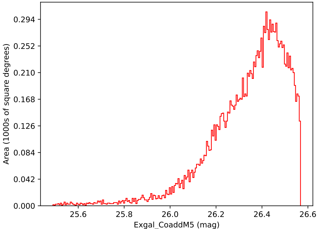
ddf_acor_sf25_lsf30_lsr10_v3.4_10yrs WFD i band: Exgal_CoaddM5
