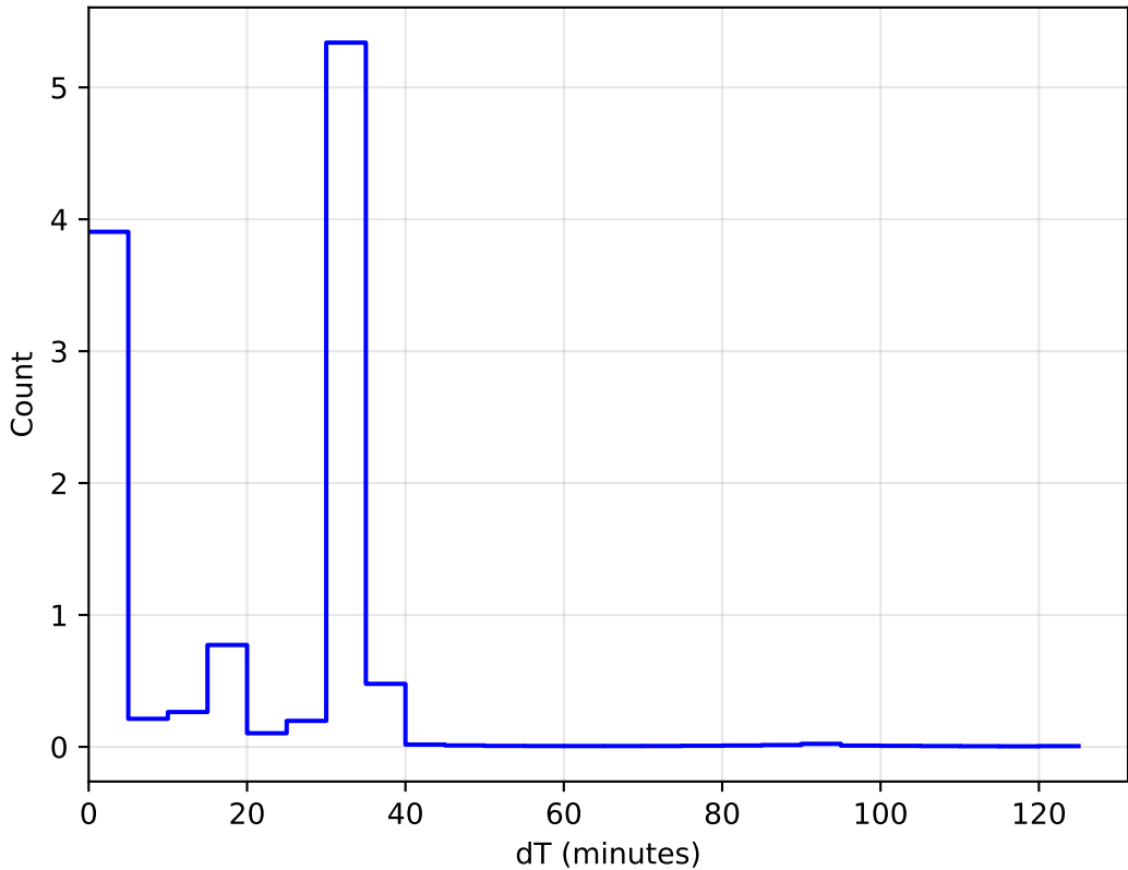
ddf_acor_sf25_lsf30_lsr10_v3.4_10yrs WFD: DeltaT Histogram 1e6
